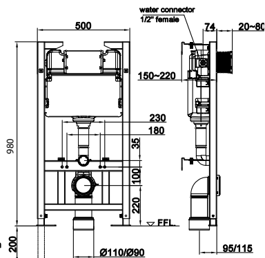
Duct mounted as front flush
