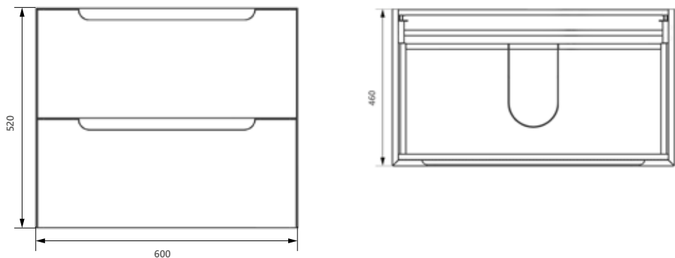
AT.620.600 Atoll 600mm wall hung unit
