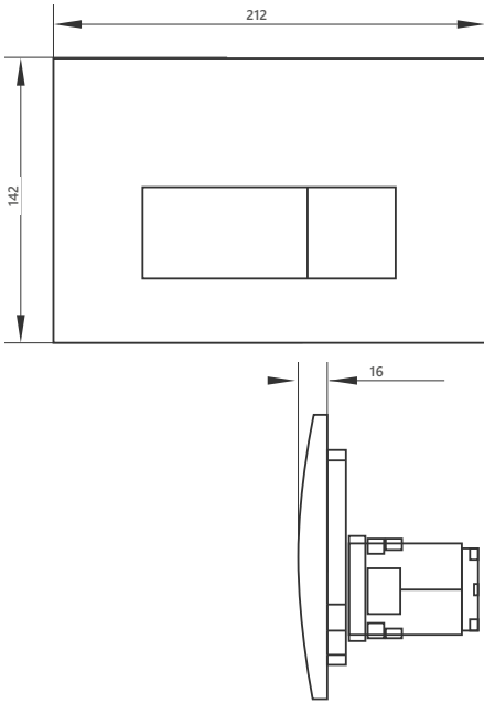
FL.760.55 Bank flush plate for use with CI.734 & CI.735
