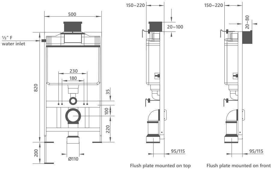
CI.735 In-wall concealed cistern with adjustable pipe length
