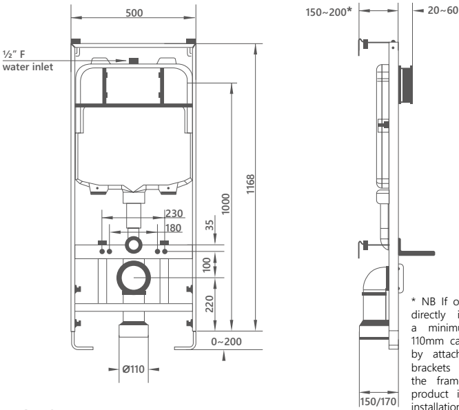
CI.734 Short concealed cistern with frame
