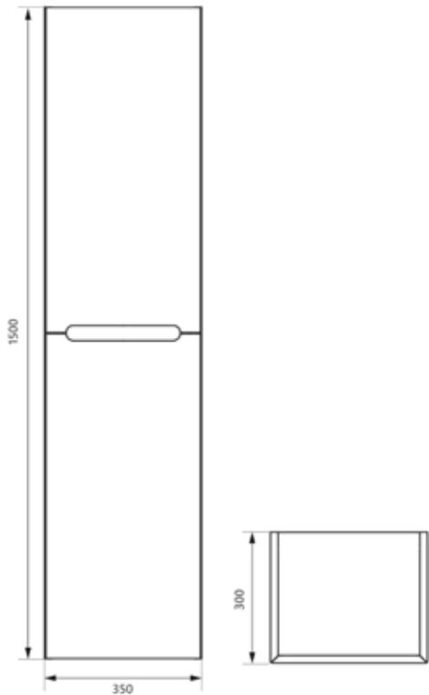
AT.650.1500 Atoll 1500mm wall hung cabinet
