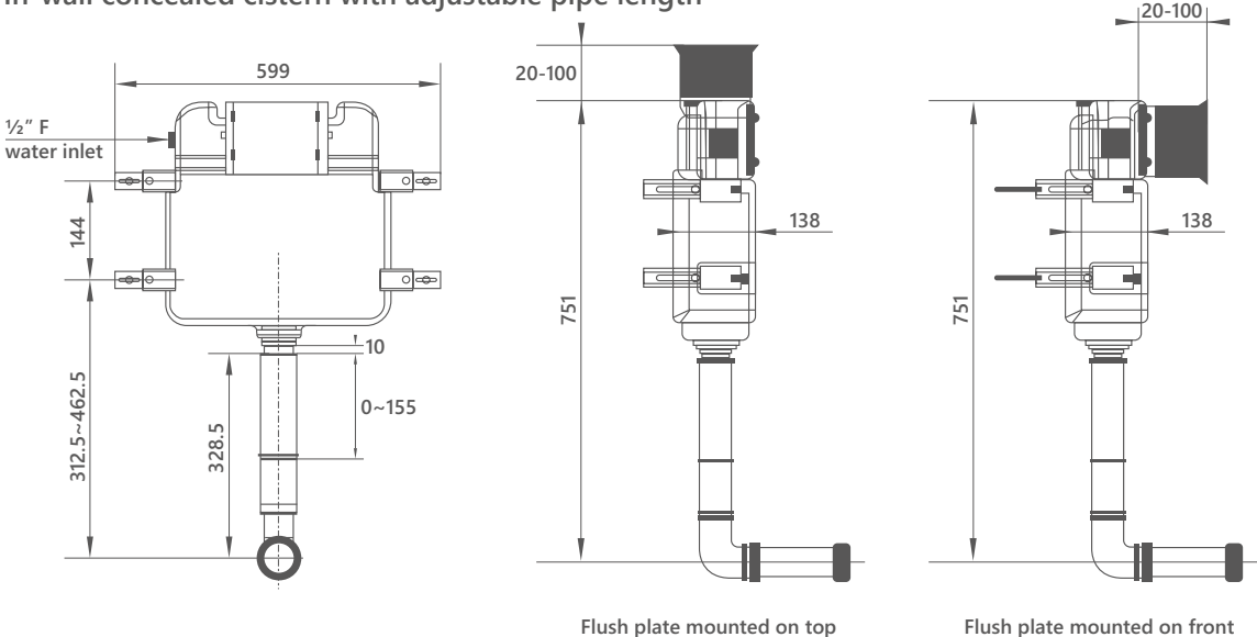
CI.735 In-wall concealed cistern with adjustable pipe length
