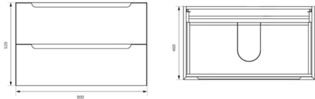
AT.620.800 Atoll 800mm wall hung unit
