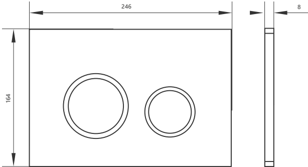
FL.760.66 Halo flush plate for use with CI.732
