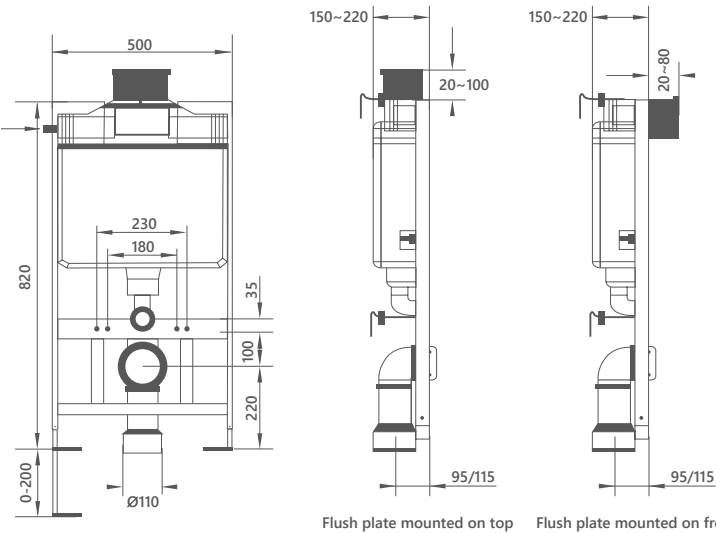
CI.734 Short concealed cistern with frame Adjustable height from 820 - 1020mm
