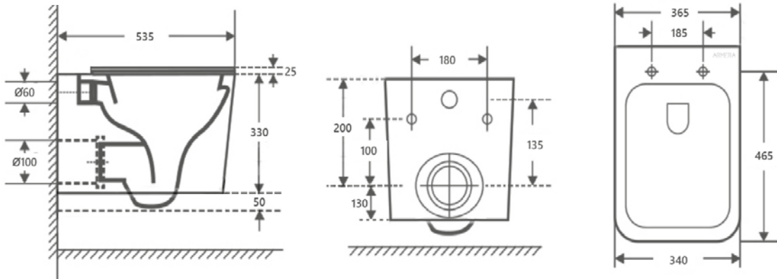
AN.713 - Anthem Wall Hung WC with seat
