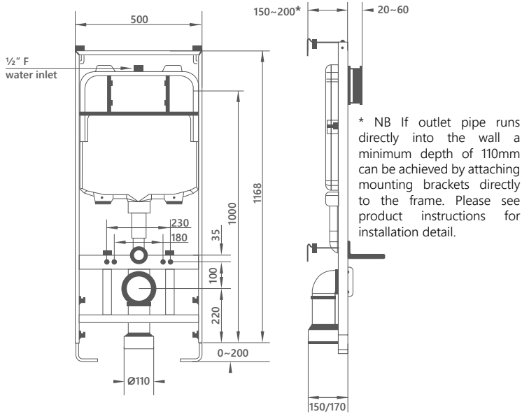
CI.733 Mid height concealed cistern with frame Adjustable height from 980 - 1180mm
