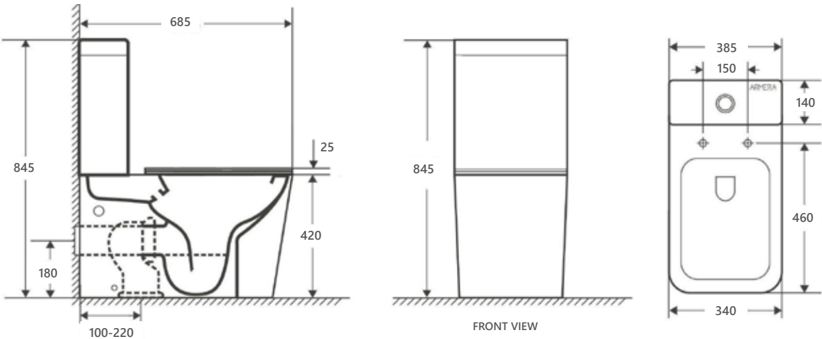
AN.712 - Anthem Back to wall WC with seat
