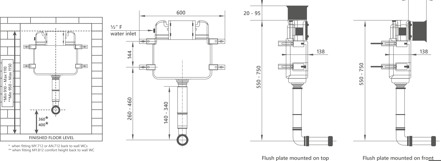
CI.735 In-wall concealed cistern with adjustable pipe length
