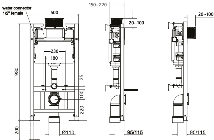
CI.735 In-wall concealed cistern with adjustable pipe length
